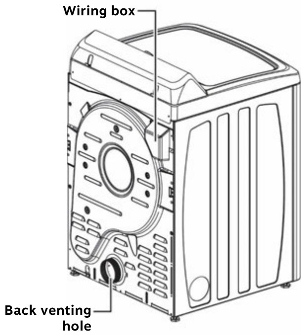
ELECTRIC DRYER
